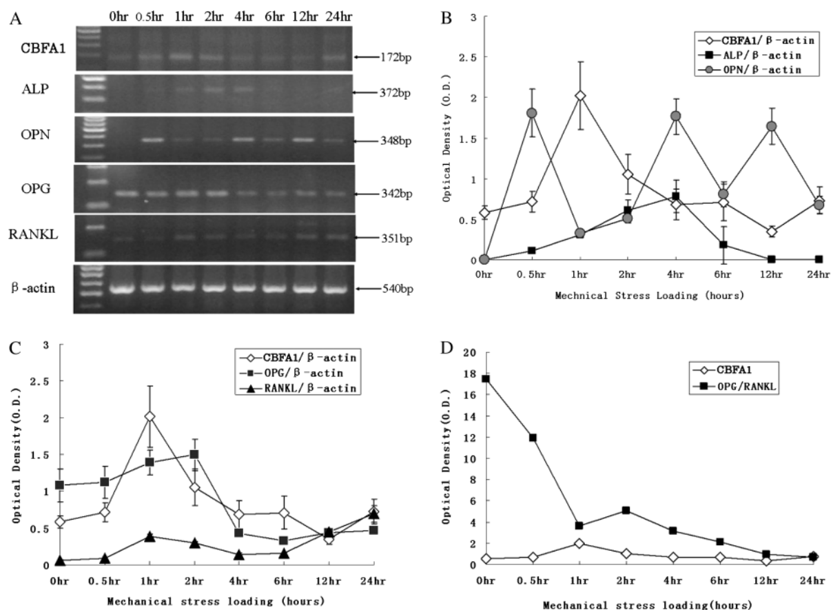
Figure 1 Effect of mechanical stress on expressions of core binding factor 1 (CBFA1), alkaline phosphatase (ALP), osteopontin (OPN), osteoprotegerin (OPG), and receptor activator nuclear factor kappa B ligand (RANKL) in human periodontal ligament (PDL) cells estimated by reverse transcription–polymerase chain reaction (PCR). The sizes of the PCR products were compared with a 100 bp DNA ladder (left lane; A). Human PDL cells were harvested at 0, 0.5, 1, 2, 4, 6, 12, and 24 hours, respectively, after mechanical stress loading. Each product was normalized with that of \beta -actin from the same template and shown as a ratio (B, C, and D). Unstretched cells (lane 0 hour) exhibited marginally detectable levels of CBFA1 messenger mRNA (mRNA). These levels were increased after 0.5 hours of intermittent applied mechanical load and reached their peak at 1 hour. After 2 hours, the level of CBFA1 began to decline and returned to an unstretched level after 6 hours (A, B, and C). At the same time, ALP mRNA expression was obvious after being stretched for 2 hours and reached its peak at 4 hours (A and B). The expression of OPN was more complicated with three peaks at 0.5, 4, and 12 hours, respectively (A and B). The level of OPG declined after 4 hours of mechanical stress loading, while that of RANKL was upregulated with the application of mechanical force (A and C). The changes of both ALP and OPG were retarded compared with that of CBFA1: the expression trendline of ALP was similar to that of CBFA1 but retarded, while OPG decreased significantly after the CBFA1 fastigium. RANKL had the same changing tendency as CBFA1 (A, B, and C). The ratio of OPG:RANKL was downregulated during the first hour after mechanical stress loading, which was opposite to the changing tendency of CBFA1 (D). Experiments were repeated three times with similar results ( n = 3 ).
